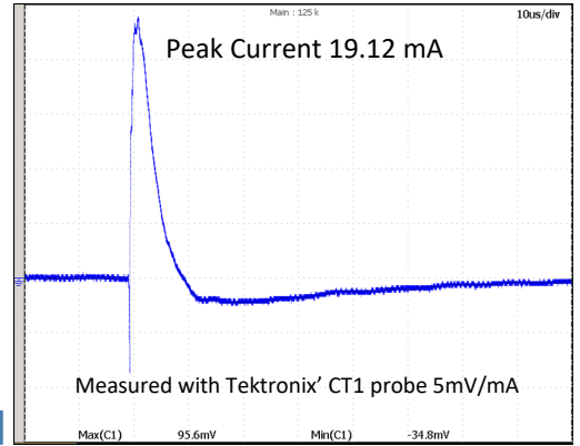
Soldering Tip Current—No Filter
