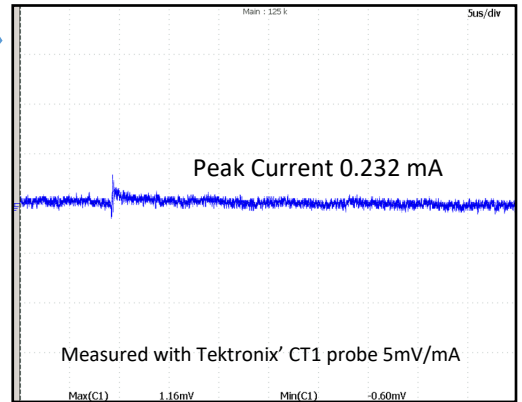
Soldering Tip Current with Soldering Filter
