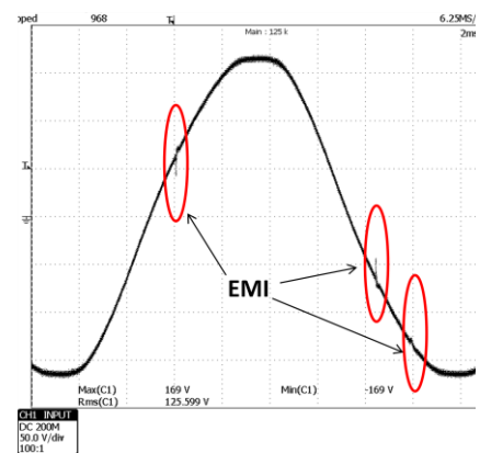
Noise on AC Line
